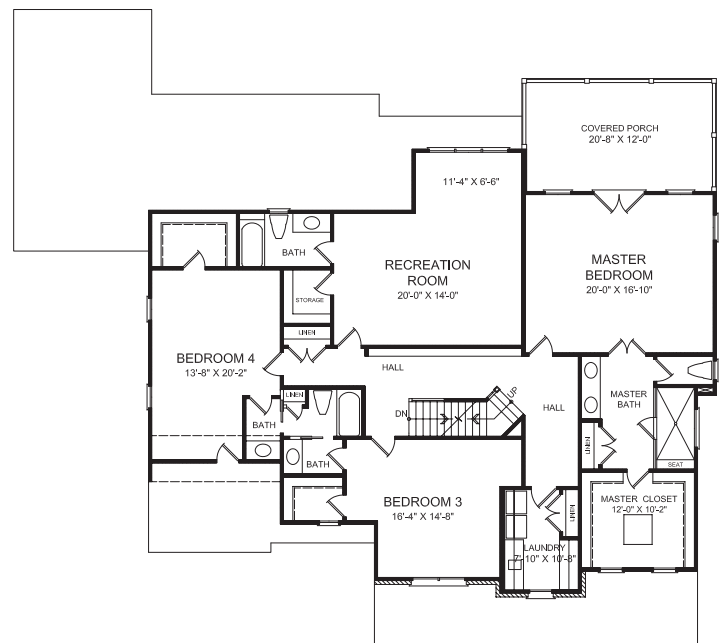
SECOND FLOOR
